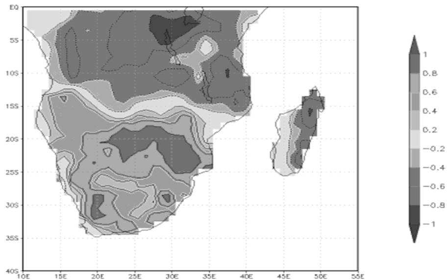
Figure 19: EOF2 October-April Normalized GPCC Rainfall, 1986-2003
