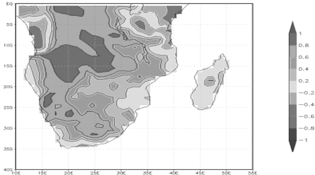
Figure 18: EOF1 October-April Normalized GPCC Rainfall, 1986-2003
