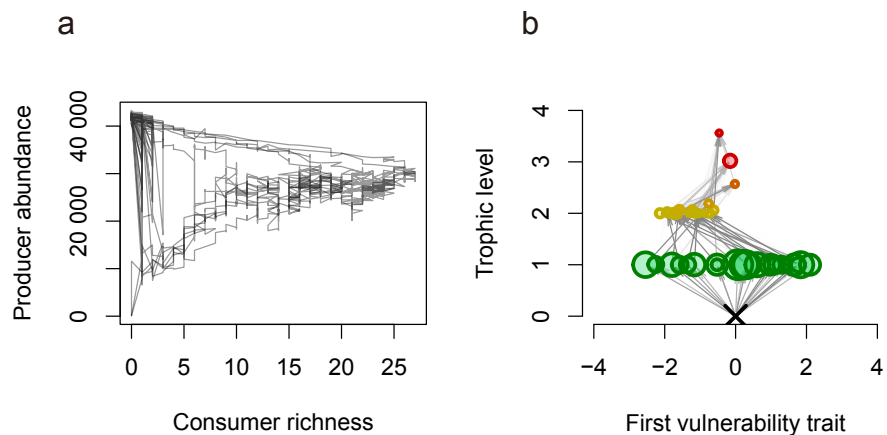
Fig. S4. Robustness with respect to increased abundance of the external resource, N_R = 9,000 . (a) The curves show the time course of consumer richness and producer abundance obtained from three independent model runs. (b) Circles represent species, with their areas being proportional to the species' abundance, their colors indicating the species' trophic level, and their horizontal positions indicating the species' first vulnerability trait. The cross at trophic level 0 represents the external resource. Arrows indicate trophic links, with darker color indicating stronger interactions. The community's overall behavior remains similar, except for a prolonged duration of the HTL state.
