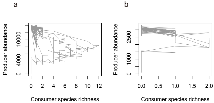
Fig. S7. Robustness with respect to introducing handling times, leading to a nonlinear functional response. We consider a Holling-type-II functional response with an attack rate of 1 and different handling times, (a) h = 1/8,000 and (b) h = 1/800 . Curves show the time course of consumer richness and producer abundance obtained from a single model run. If handling times are sufficiently small (a), we observe the same evolutionary cycles as with the linear response.
