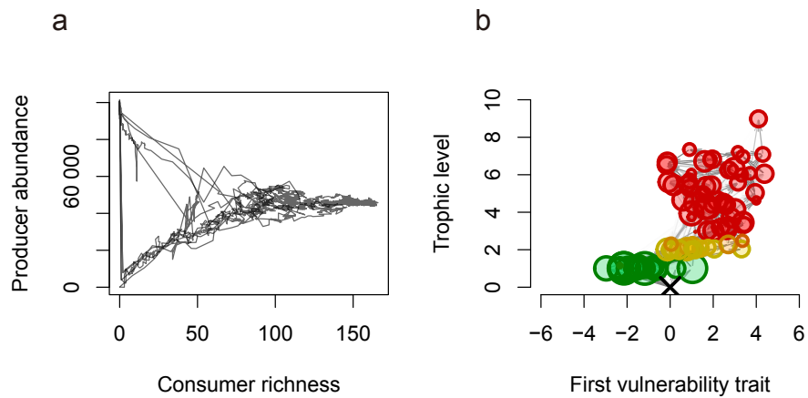
Fig. S3. Robustness with respect to increased trophic efficiency, a = 0.9 . (a) The curves show the time course of consumer richness and producer abundance obtained from a single model run. (b) Circles represent species, with their areas being proportional to the species' abundance, their colors indicating the species' trophic level, and their horizontal positions indicating the species' first vulnerability trait. The cross at trophic level 0 represents the external resource. Arrows indicate trophic links, with darker colors indicating stronger interactions. The community's overall behavior remains the same, except for higher trophic levels and larger species richness.
