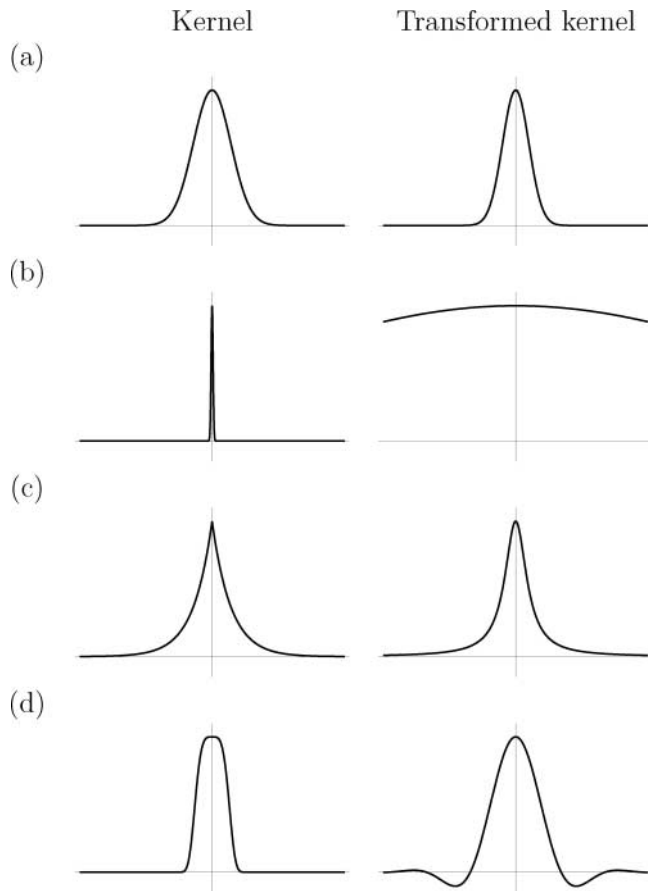
Fig. 2. Examples of different homogeneous competition kernels a (left column) and their Fourier transforms \tilde{a}(z) (right column). The examples shown focus on symmetric kernels, whose Fourier transforms are symmetric functions with real values. Interpretation of the values \tilde{a}(z) for continuous z is analogous to that of the eigenvalues of the Jacobian matrix A for a discrete set of species (Box 1): the continuous-coexistence solution under a competition kernel a is dynamically stable against a small perturbation of frequency z if and only if \tilde{a}(z) > 0 , so it is dynamically stable against all small perturbations if and only if \tilde{a}(z) > 0 holds for all z . (a) The Fourier transform of a Gaussian kernel is a Gaussian function with inverse width: because \tilde{a}(z) > 0 holds for all z , all such kernels are positive-definite. (b) The Fourier transform of a very narrow Gaussian kernel is a very wide Gaussian function. In the biologically unrealistic limit of an infinitely narrow Gaussian kernel (known as a Dirac delta function), the Fourier transform is therefore flat. (c) The Fourier transform of a kinked kernel also goes to zero for large z , but does so more slowly than for a Gaussian kernel with equal standard deviation. (d) The Fourier transform of a platykurtic kernel, which is more ‘box-like’ than a Gaussian kernel, also goes to zero for large z , but is negative for a range of intermediate frequencies z , implying dynamical instability against small perturbations of those frequencies.
