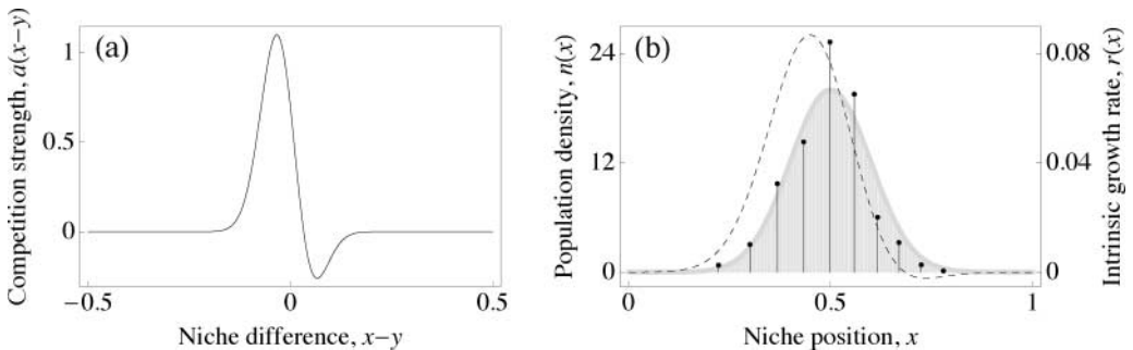
Fig. 4. Coexistence under an analytic competition kernel. (a) The competition kernel a is obtained as a(x - y) = e^{-225(x - y)^2} (1 - 30(x - y))/\sqrt{2} . One can show that this kernel is positive definite. Note that the kernel does not attain its maximum at zero niche difference, and that the species interactions described by this kernel are not purely competitive. (b) The distribution r of intrinsic growth rates (dashed curve) is constructed so as to yield the continuous-coexistence solution n(x) = \exp(-(x - 0.5)^2/0.02) (grey curve and area) in conjunction with this particular competition kernel. This is achieved by inserting the kernel and the desired continuous-coexistence solution into equation (2). We perturb this distribution r with a small and very narrow perturbation at x = 0.5 . The outcome is obtained by following the dynamics of equation (1), approximated by 400 equidistant species, until equilibrium is reached, from a uniform initial condition. Even though the perturbation is small, it completely collapses continuous coexistence, leaving only ten discrete, more-or-less evenly spaced surviving species (vertical lines).
