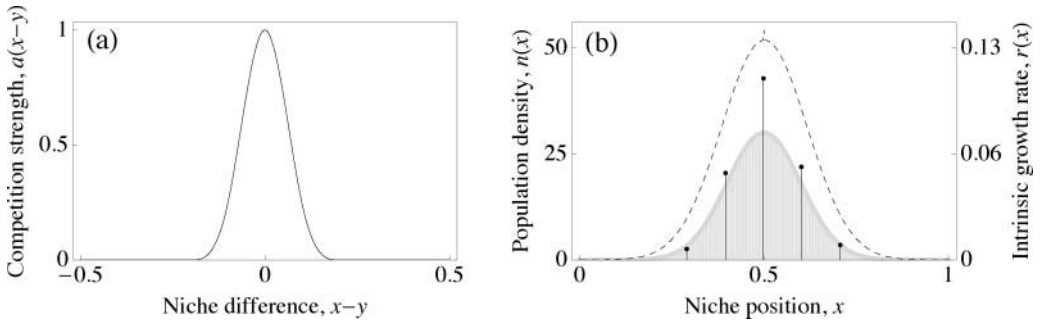
Fig. 5. Coexistence under a smooth non-analytic competition kernel. (a) The competition kernel a is obtained as a(x-y) = \int u(x-z)u(y-z) dz with a resource-utilization function u that equals u(x) = 1 - |10x| for x \leq 1/10 and zero otherwise. The construction of this kernel as an overlap kernel guarantees its positive definiteness. It is smooth enough to be twice differentiable, but not smooth enough to be analytic, as its third derivative is already discontinuous. (b) The distribution r of intrinsic growth rates (dashed curve) is constructed so as to yield the continuous-coexistence solution n(x) = \exp(-(x-0.5)^2/0.02) (grey curve and area) in conjunction with this particular competition kernel, just as in Fig. 4. We perturb this distribution r with a small and very narrow perturbation at x = 0.5 (tiny peak at the top of the dashed curve). The outcome is obtained by following the dynamics of equation (1), approximated by 400 equidistant species, until equilibrium is reached, from a uniform initial condition. Even though the perturbation is small, it completely collapses continuous coexistence, leaving only five discrete, more-or-less evenly spaced surviving species (vertical lines). Observe that the distance between neighbouring surviving species roughly equals twice the standard deviation of the competition kernel.
